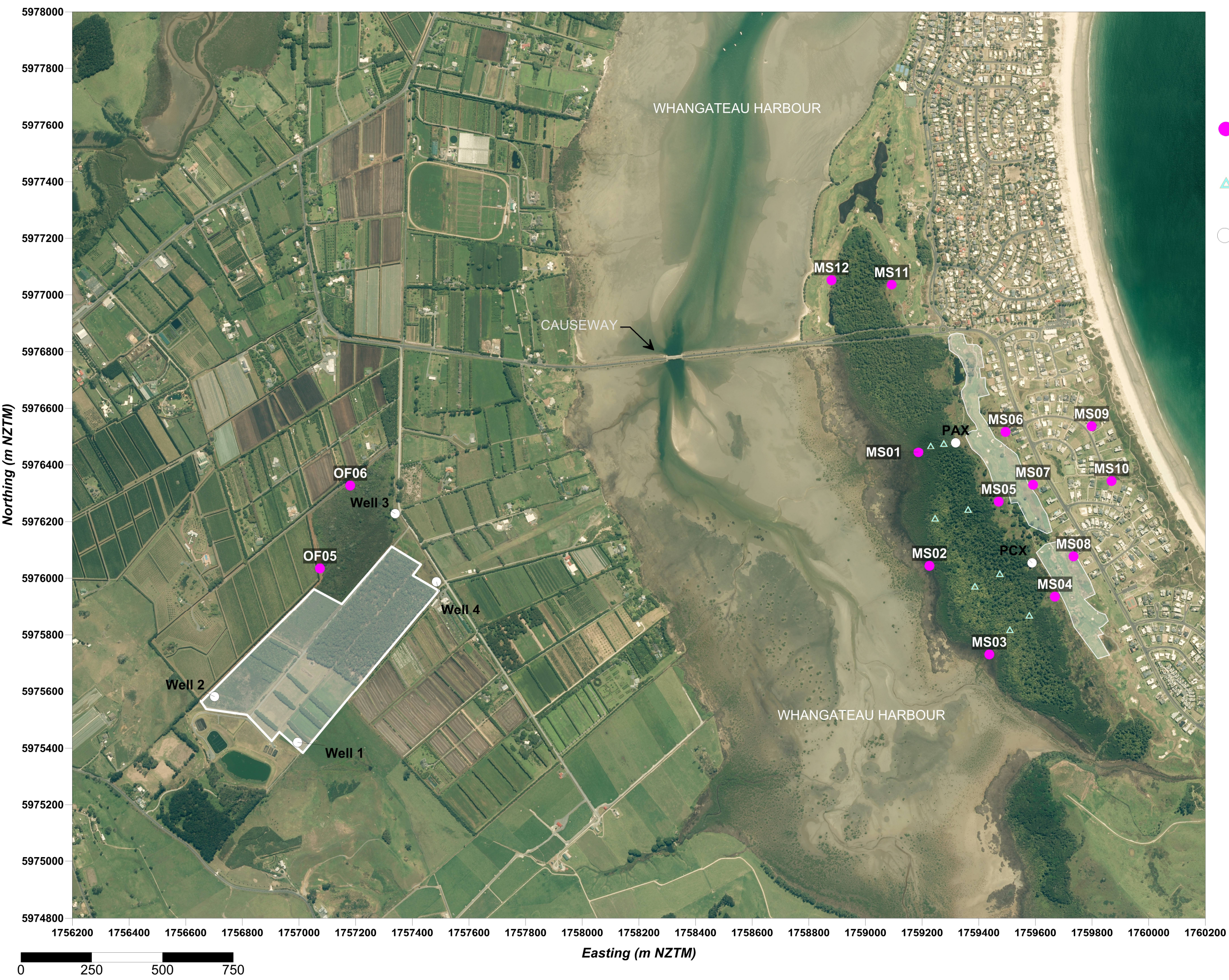
FIGURE 1: PLANNED GROUNDWATER BORE AND HAND AUGER LOCATIONS
